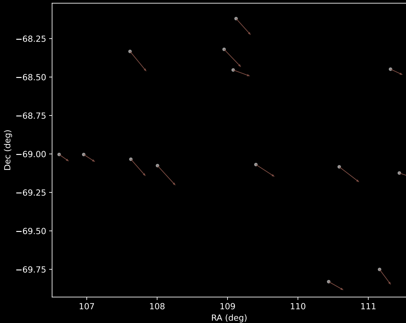
GALAH DR4 Cluster 10 Proper Motion Vectors (n=14)
