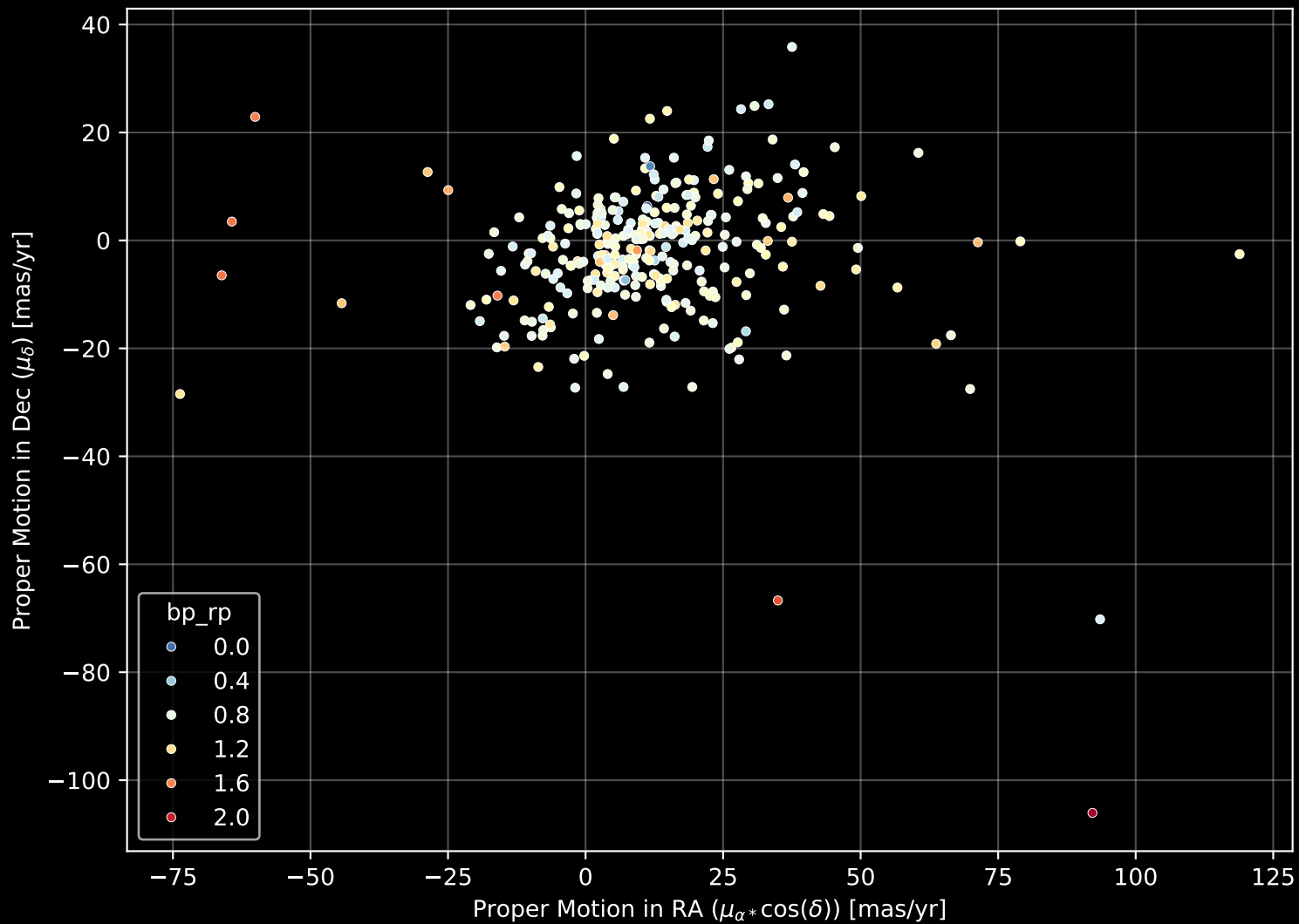
GALAH DR4 Field: [7047] Proper Motion Diagram (n= 311)
