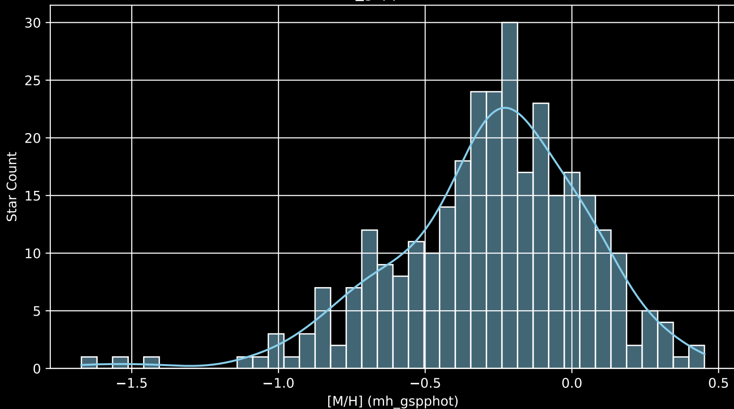
GALAH DR4 Field: [7047] [M/H] (mh_gspphot) (n= 311)
