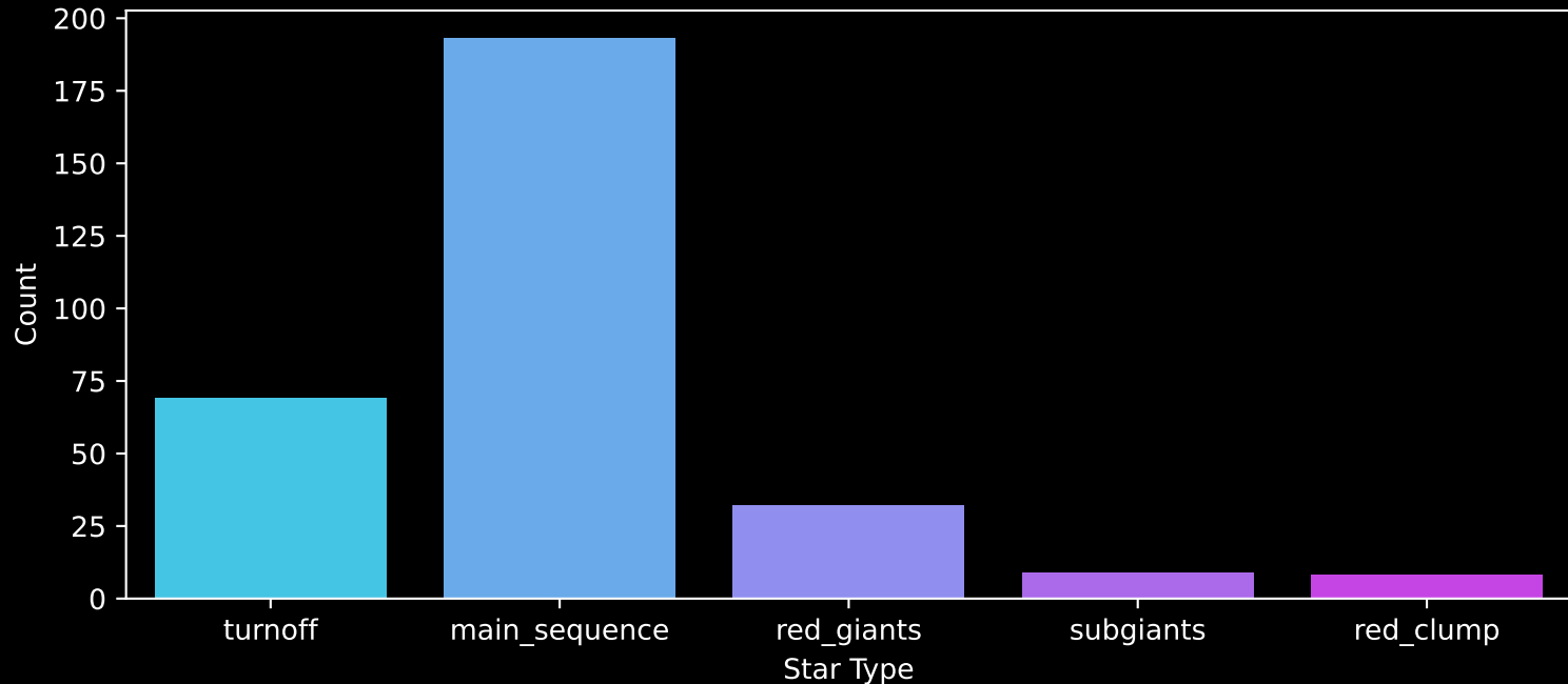
GALAH DR4 Field: [7047] Count plot of Star Type
