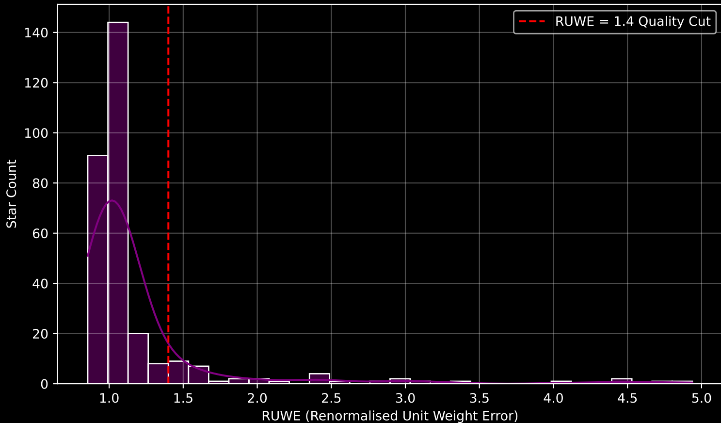
GALAH DR4 Field [7047] RUWE Distribution (n= 300)
