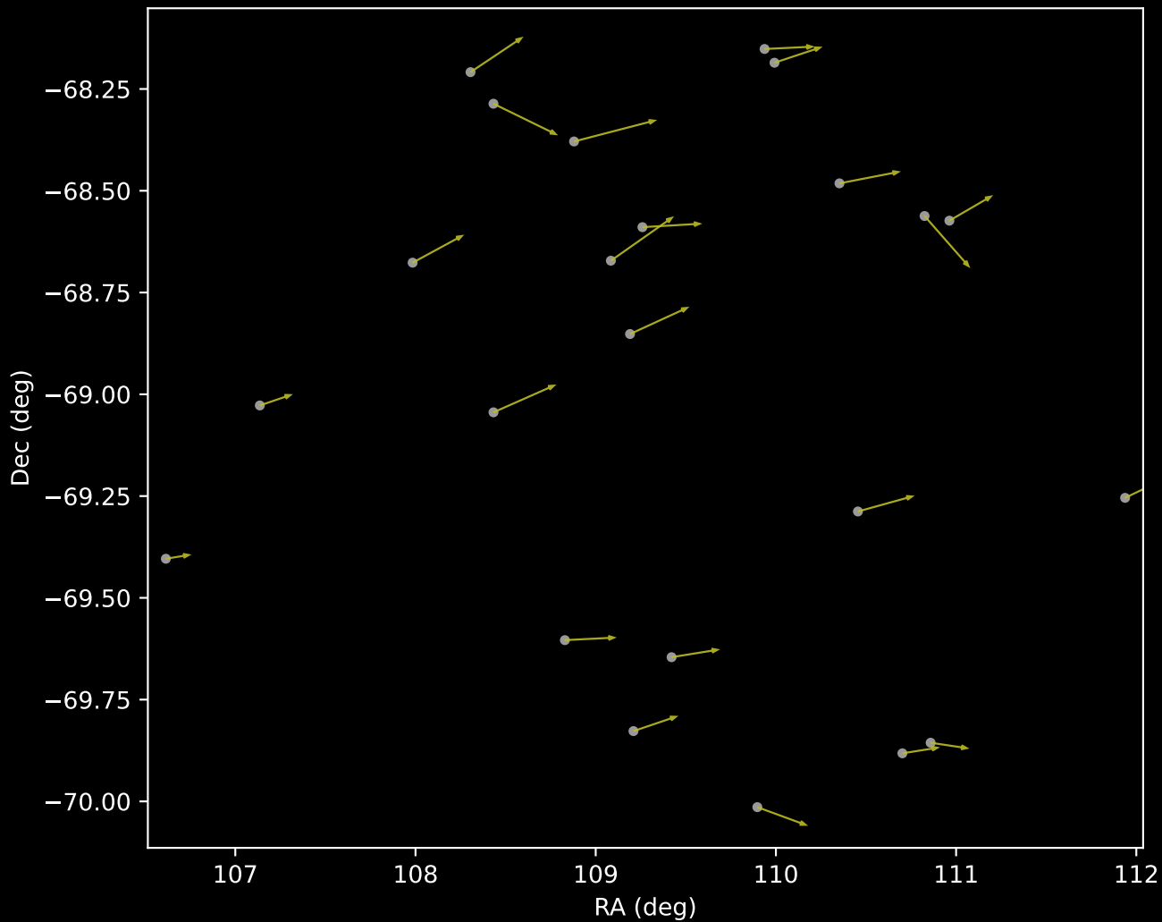
GALAH DR4 Cluster 16 Proper Motion Vectors (n=23)
