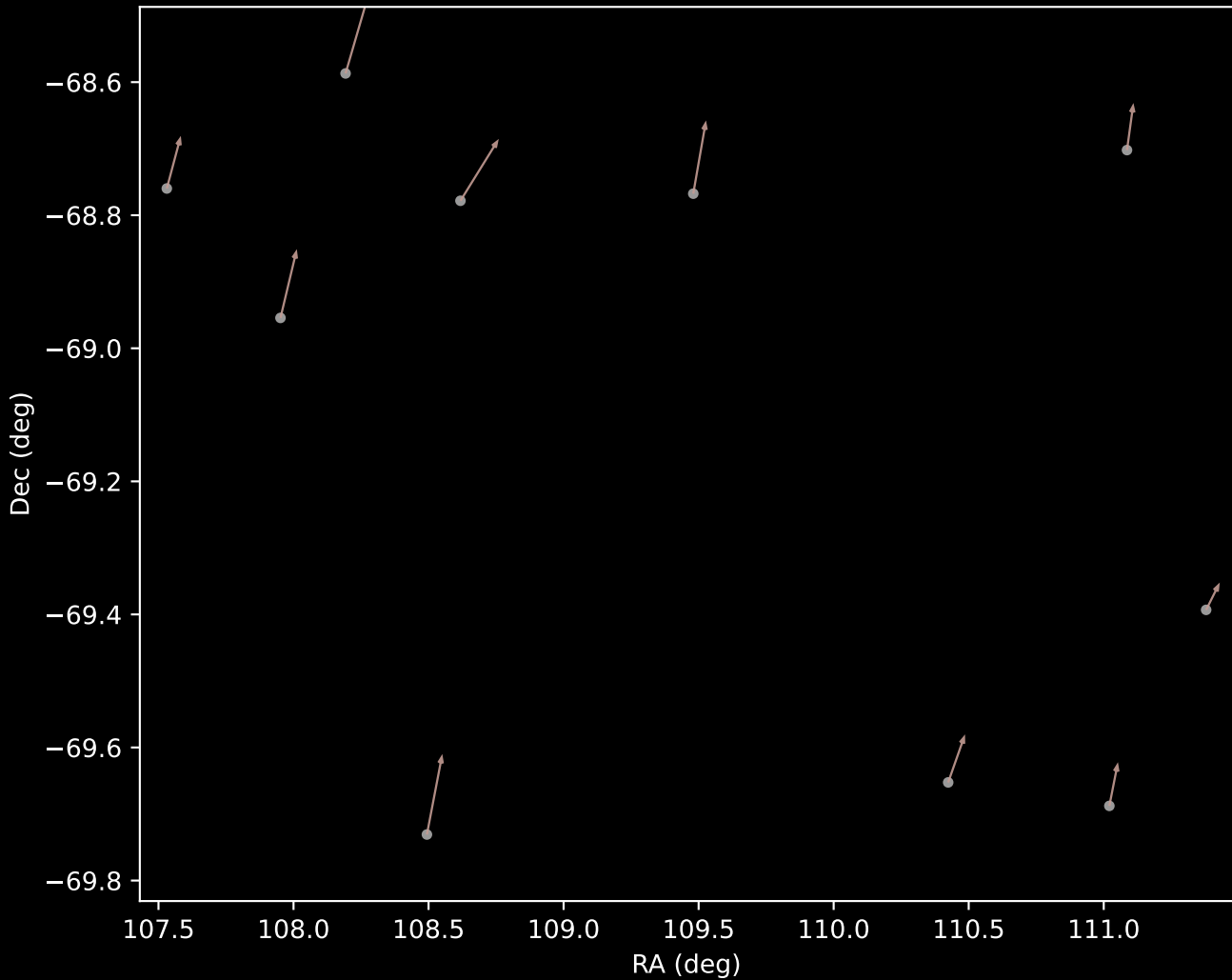
GALAH DR4 Cluster 11 Proper Motion Vectors (n=10)
