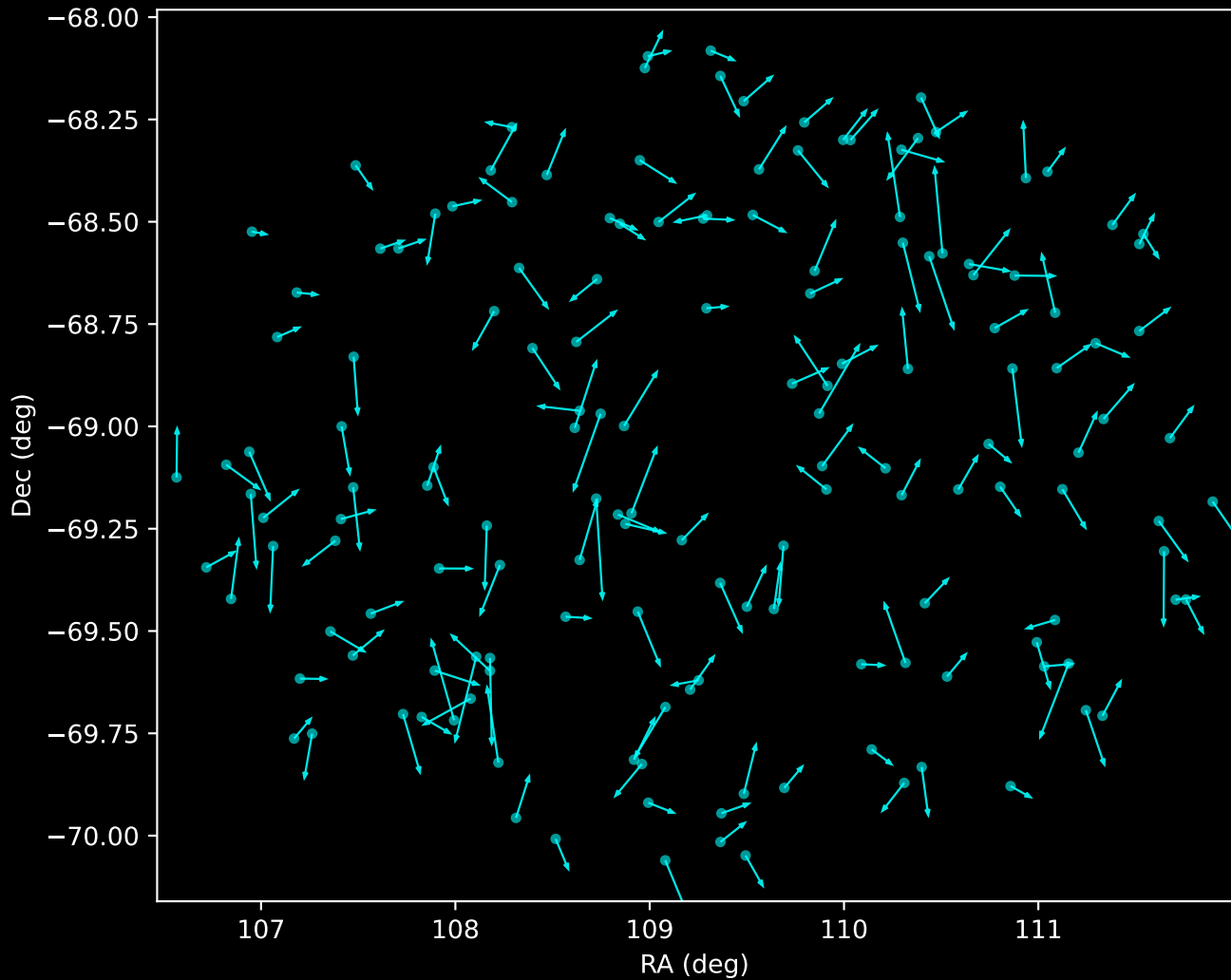
GALAH DR4 Noise Stream Proper Motion Vectors (n=157)
