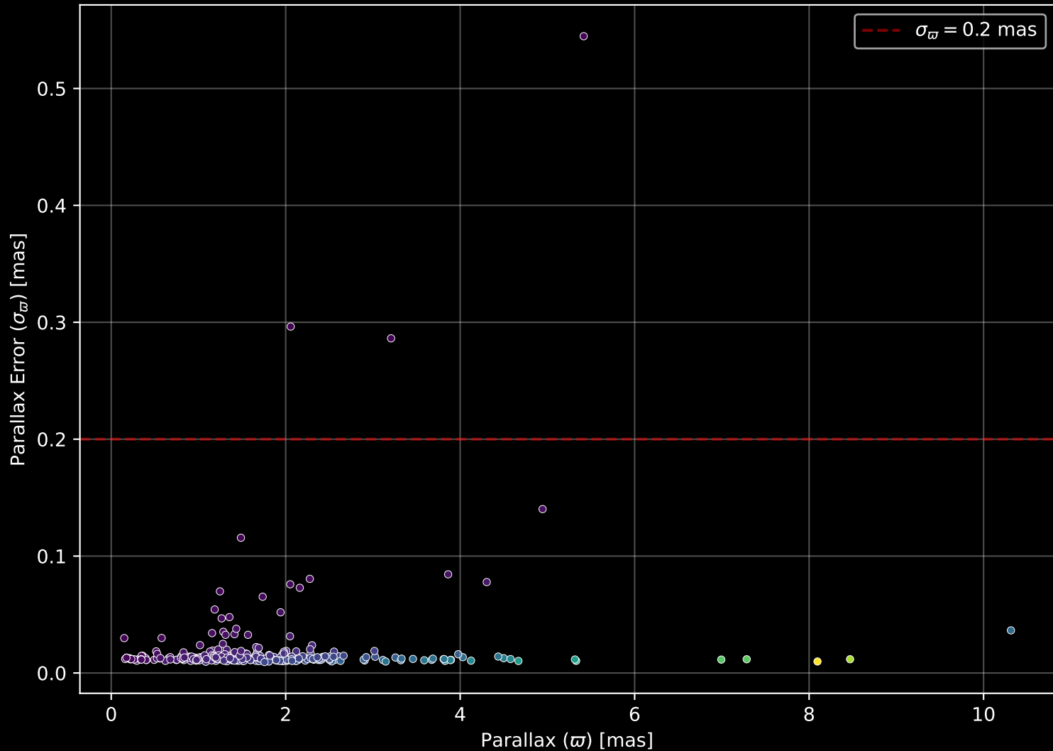
GALAH DR4 Field: [7047] Parallax Quality (n= 311)
